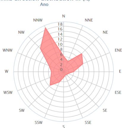
Wind direction distribution in (%)
